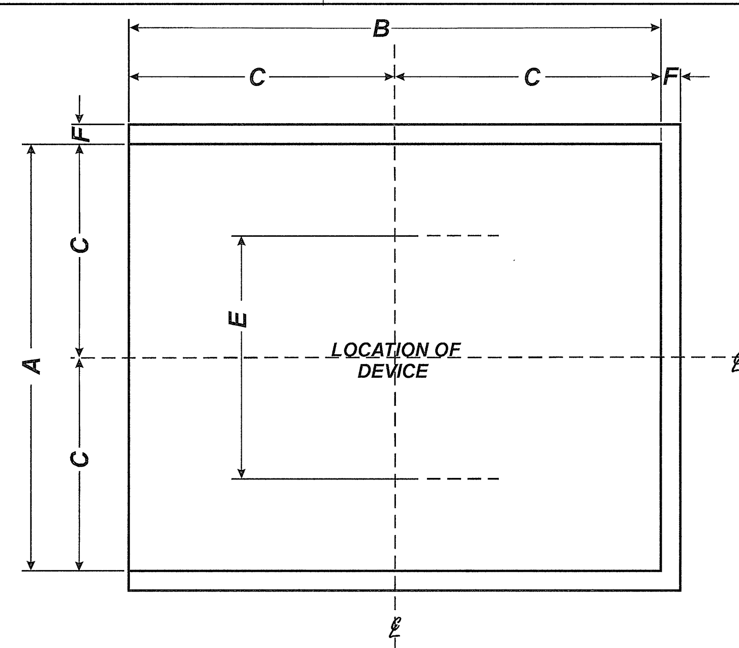
DISTINGUISHING FLAG - SCALE 1" = 1'-0" FOR 4'-4" X 5'-6" FLAG
